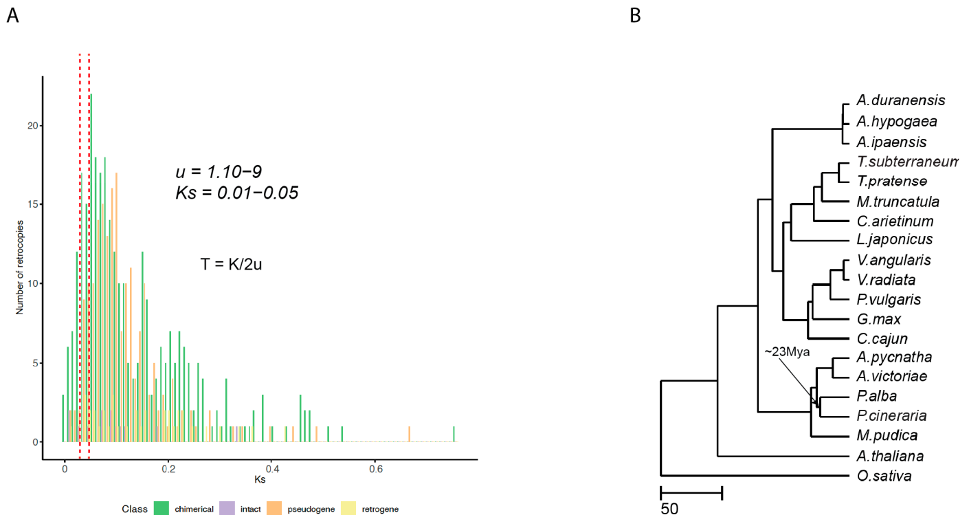
Figure 5. The timing of chimerical retrogene generation in P. cineraria . (A) Ks distribution of the different classes of retrogenes. The red dotted lines around Ks = 0.01-0.05 highlights the initial amplification. (B) Ultrametric tree highlighting the time of divergence of P. cineraria and P. alba , which overlaps with major amplification of chimerical retrogenes, using a mutation rate of 10^{-9} and using the formula ( T = k/2u ).
