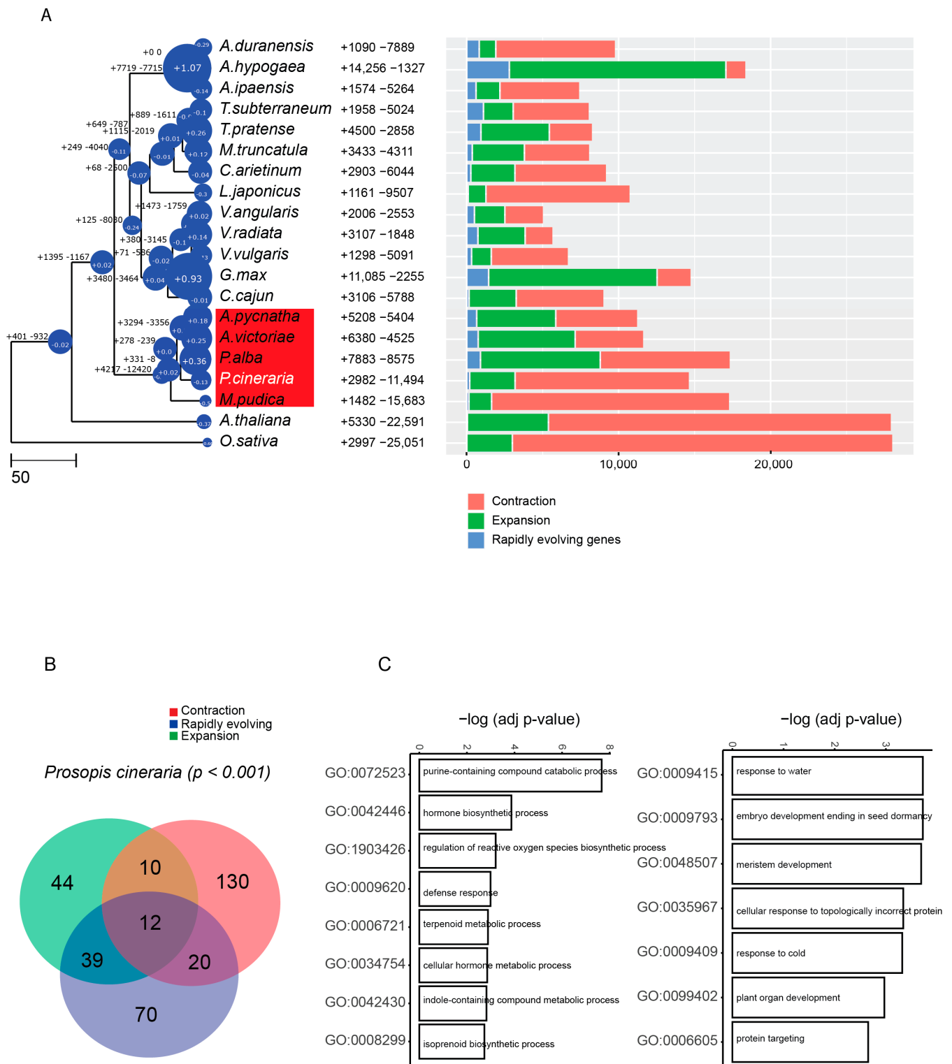
Figure 2. Genome evolution of P. cineraria . (A) Ultrametric tree of 18 legumes, including the mimosoid clade (highlighted by red box) and the two outgroups A. thaliana and O. sativa . CAFÉ analysis depicts total number of expanded and contracted gene families as well as rapidly evolving genes. The bubble on the node and leaf of the tree highlights the average expansion or contraction for each of the species, where a positive number depicts more expansion. (B) Venn diagram of top significant gene families ( p < 10^{-2} ) that are expanded or contracted in P. cineraria and under positive selection. (C) GO term enrichments of expanded gene families that are under selection ( left ) and contracted gene families under selection ( right ).
