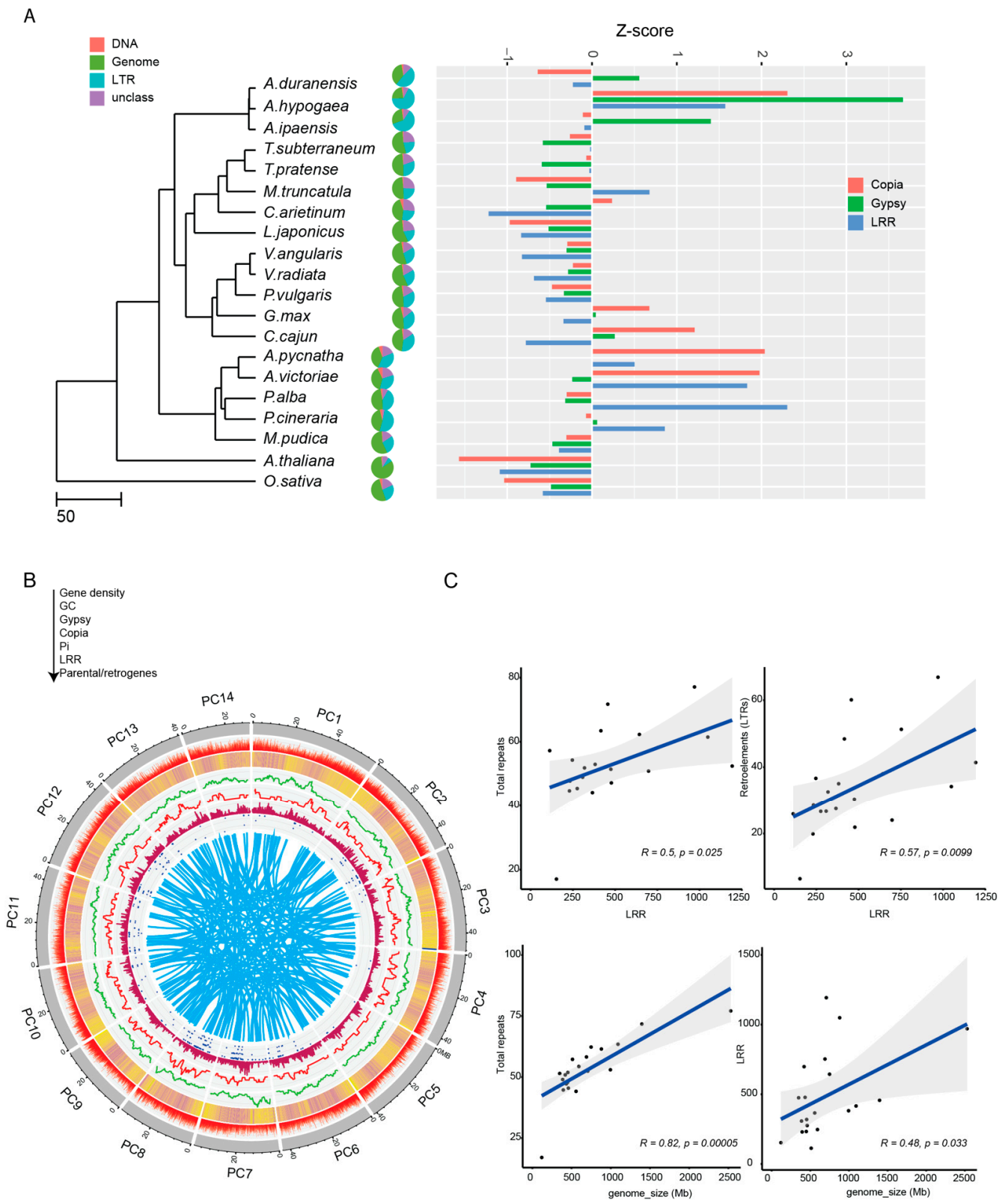
Figure 3. Comparative genome analysis of repeats, including disease resistance genes (NBS-LRR). (A) Pie chart of the percentage of DNA, LTR-retrotransposons, and unclassified repeats of the genome mapped onto the ultrametric tree. Z-score of the number of NBS-LRR, copia -like and gypsy -like
